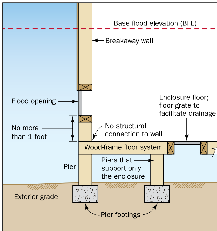
Figure 10: Above-grade enclosure supported by independent foundation
